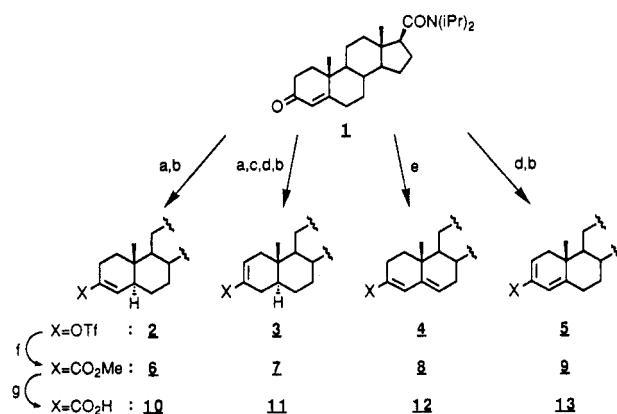
Scheme I a
