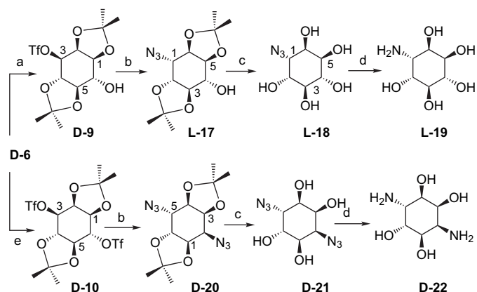
Scheme 3. (a) \text{Tf}_2\text{O} (1.1 equiv), Py, \text{CH}_2\text{Cl}_2 , -20^\circ\text{C} ; (b) \text{NaN}_3 , DMF, 70^\circ\text{C} ; (c) \text{TFA-H}_2\text{O} (4:1), rt; (d) \text{H}_2 , Pd-C, MeOH, rt; (e) \text{Tf}_2\text{O} (2.2 equiv), Py, \text{CH}_2\text{Cl}_2 , -20^\circ\text{C} .
