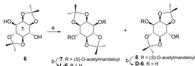
Scheme 1. ( S )- O -Acetylmandeloyl chloride, Py, 0 °C; (b) isobutylamine, MeOH, reflux.
