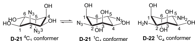
Chart 2. Conformational preferences of D-21 and D-22.
