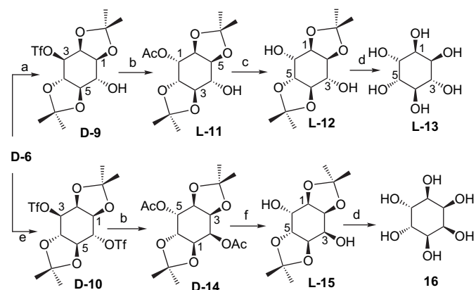
Scheme 2. (a) \text{TiF}_2\text{O} (1.1 equiv), Py, \text{CH}_2\text{Cl}_2 , -20^\circ\text{C} ; (b) KOAc, DMA, 70^\circ\text{C} ; (c) MeOH, \text{Et}_3\text{N} , reflux; (d) TFA– \text{H}_2\text{O} (4:1), rt; (e) \text{TiF}_2\text{O} (2.2 equiv), Py, \text{CH}_2\text{Cl}_2 , -20^\circ\text{C} ; (f) NaOMe, MeOH, reflux.
