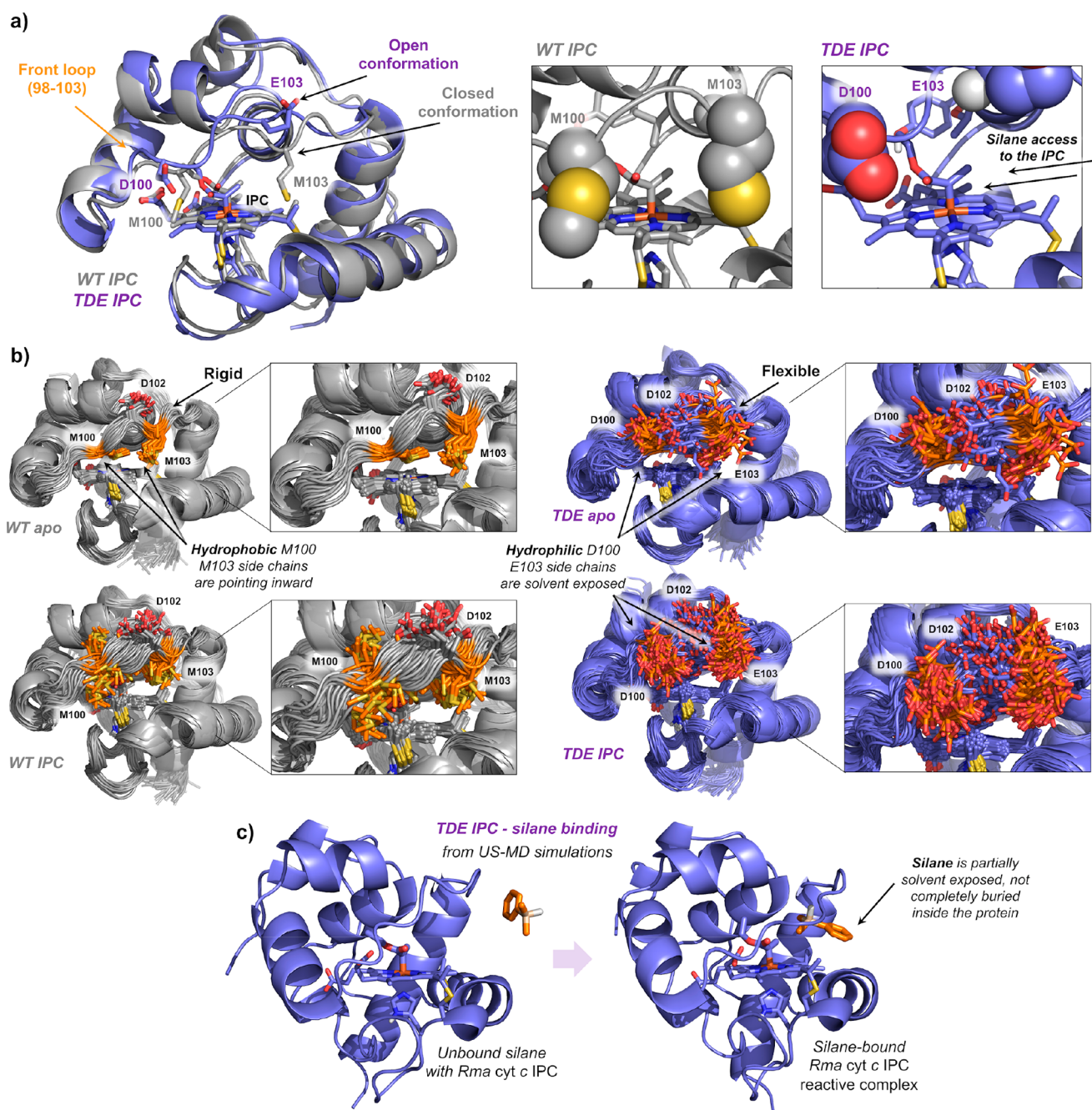
Figure 2. (a) Representative snapshots obtained from MD simulations of IPC bound in wild-type Rma cyt c (gray) and the Rma TDE variant (purple). Front loop M100/D100 and M103/E103 residues are represented in space filling format. Hydrophobic methionines (M100 and M103) close the substrate channel in wild-type Rma cyt c, but mutations M100D and M103E introduce hydrophilic residues that are exposed to the solvent in Rma TDE along the MD simulations, allowing an easier access of the silane substrate to interact with the IPC. V75T creates new key H-bond with Y71 that induces a more hydrophobic environment for the IPC intermediate. (b) Overlay of 50 snapshots (every 10 ns) obtained from 500 ns MD simulations for wild-type Rma cyt c and Rma TDE variants in its apo and IPC-bound states. Residues mutated in the front loop (original M100 and M103 in WT, and D100 and E103 in TDE variant) are shown in orange. Insets highlight the flexibility acquired by the front loop due to newly introduced mutations (going from "WT apo" to "TDE apo") and the formation of the IPC (going from "WT apo" to "WT IPC" and "TDE apo" to "TDE IPC", respectively). Corresponding RMSF analysis are reported in Figure S8. (c) Representative snapshots of silane binding to Rma TDE IPC in a catalytically relevant pose obtained from umbrella sampling MD simulations.
