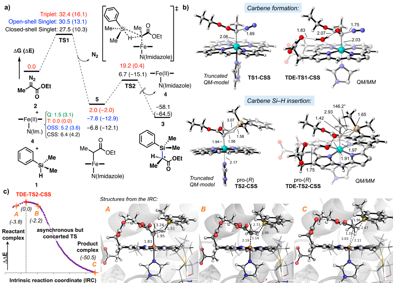
Figure 1. (a) Computed reaction pathway for carbene Si–H insertion reaction between PhMe 2 SiH 1 and Me-EDA 2 catalyzed by a model imidazole-ligated iron porphyrin (truncated DFT model). Results with three iron electronic states are given. The calculated intrinsic electronic and Gibbs free energies are given in kcal·mol -1 . Gibbs free energies do not consider the formation of substrate–substrate or enzyme–substrate reactant complexes, thus neglecting the stabilizing interactions that overcome the unfavorable -T\Delta S term of a bimolecular reaction (usually about 12 kcal·mol -1 in the free energies). (b) Optimized geometries for the lowest in energy TS1-CSS and TS2-CSS obtained from truncated QM and QM/MM models (only atoms included in the QM region are shown for clarity). (c) Intrinsic reaction coordinate (IRC) calculation for the lowest energy Si–H carbene insertion transition state (TDE-TS2-CSS) calculated using QM/MM (atoms included in the QM region are shown in ball and stick format). Relative electronic energies are given in kcal·mol -1 . Key distances and angles are shown in Å and degrees.
