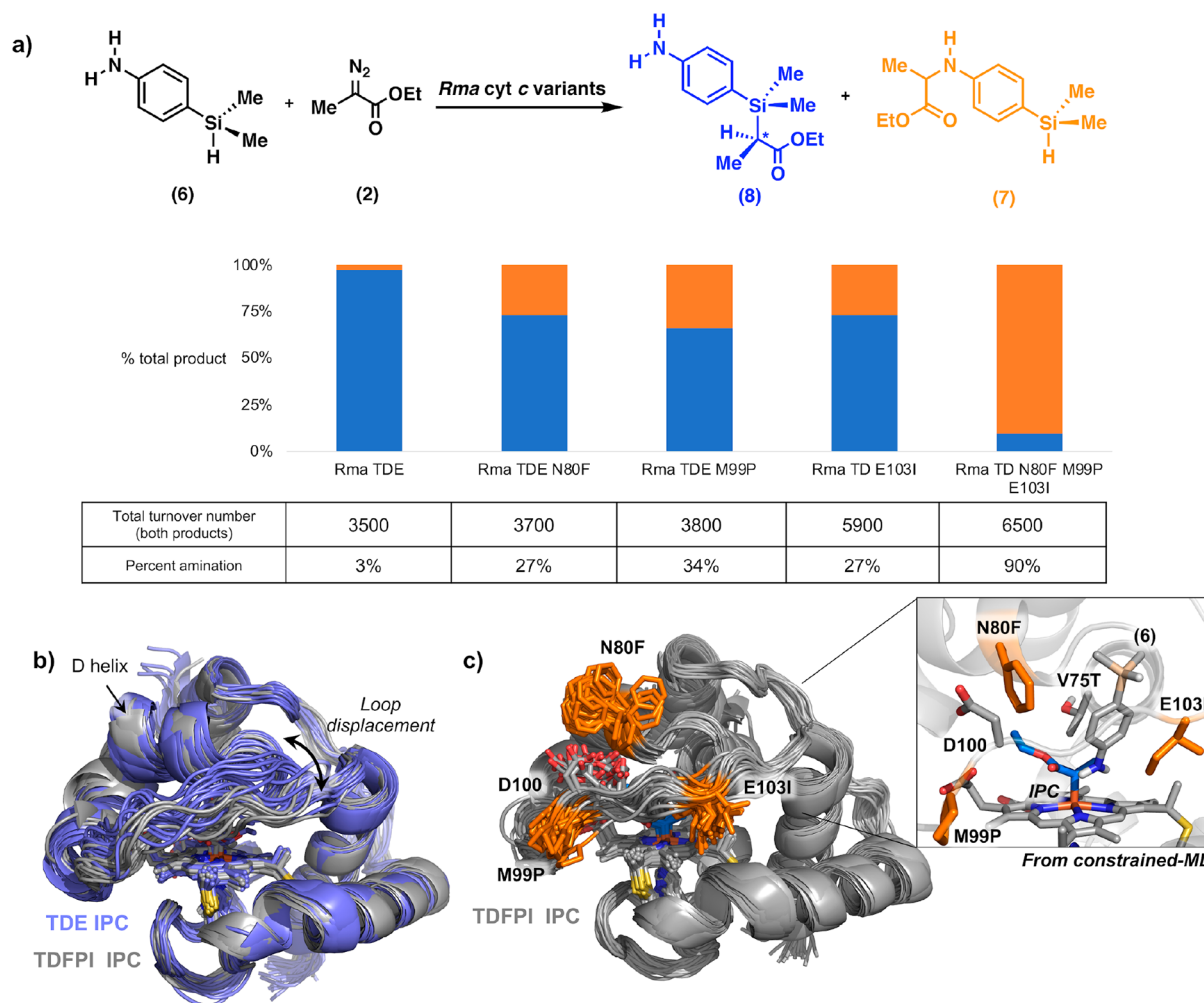
Figure 4. (a) Site saturation mutagenesis of Rma TDE for chemoselective amination over Si–H carbene insertion using p -dimethylsilylaniline 6 and diazo compound 2 . Reactions were performed with heat-treated cell lysates with 1 \mu M Rma cyt c protein, 10 mM 6 , 10 mM 2 , and 10 mM sodium dithionite in M9-N buffer. Chemoselectivity was measured as the percent of amination product over total product formed and was determined by gas chromatography. Total turnover number (TTN) is defined as the combined concentration of 7 and 8 , over protein concentration. See Supporting Information for full description of the experimental procedures. (b) Overlay of different snapshots obtained from 500 ns MD trajectories of Rma TDE (purple) and Rma TDFPI (gray) IPC-bound complexes. The most important structural changes correspond to the preferred “top-open” conformation adopted by the front loop (residues 98–103) in Rma TDFPI as compared to the parent Rma TDE variant. (c) Overlay of snapshots obtained from 500 ns MD trajectory for Rma TDFPI IPC-bound complex. The mutations N80F, M99P, and E103I are highlighted in orange. Inset: Snapshot from constrained-MD simulation of Rma TDFPI IPC-bound complex with substrate 6 , showing how substrate 6 prefers to adopt a binding pose that favors amination via N-nucleophilic attack.
