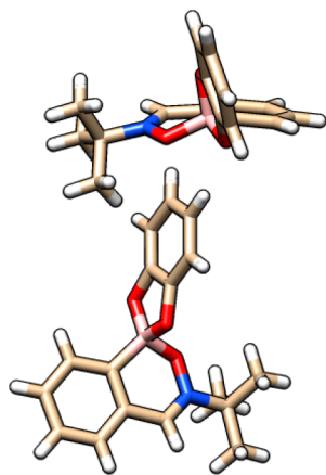
Figure 1. Crystal structure of 3, grown from CH 2 Cl 2 .
