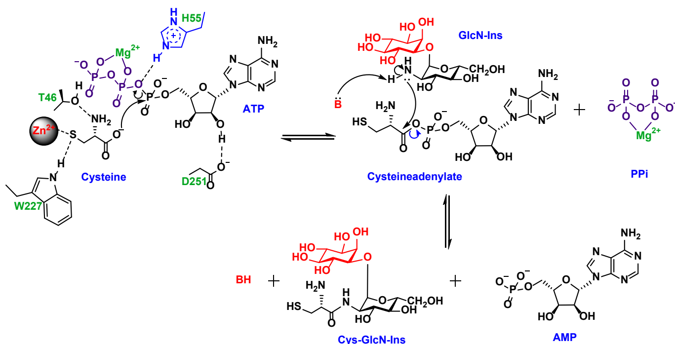
Fig. 2. Proposed enzyme mechanism of MshC.
