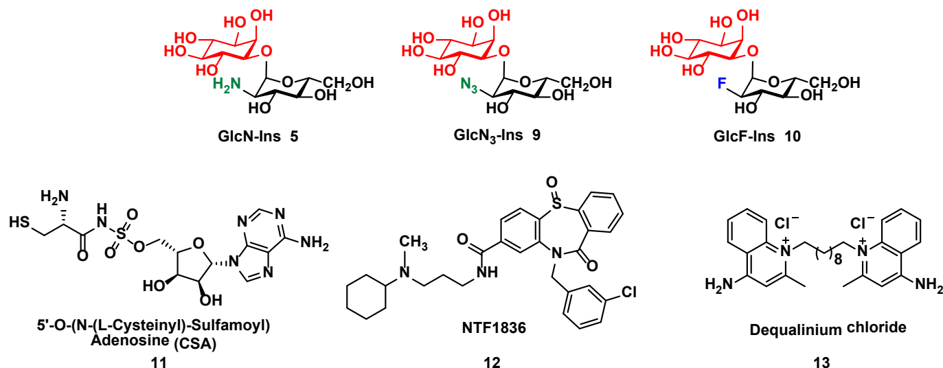
Fig. 3. Substrate for MshC ( 5 ) and analogues ( 9 , 10 ). Known inhibitors for MshC ( 11–13 ) [17,22,23].
