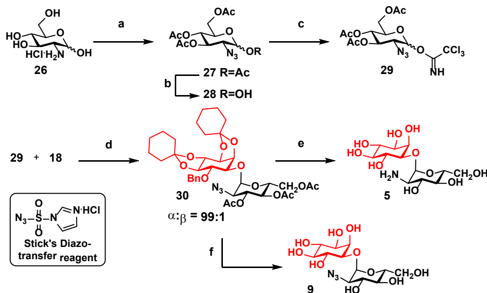
Scheme 3. Reagents and conditions: a) (i) Stick's diazo transfer reagent, \text{K}_2\text{CO}_3 , \text{CuSO}_4 \cdot 5\text{H}_2\text{O} , MeOH, RT, 3 h, (ii) \text{Ac}_2\text{O} , Pyridine, DMAP, RT, 12 h (87%); b) Ammonium acetate, DMF, RT, 12 h, (98%); c) Trichloroacetonitrile, \text{K}_2\text{CO}_3 , anhydrous DCM, 0^\circ\text{C} to RT, 16 h, (90%); d) TMSOTf, anhydrous DCM, MS-4 Å, -20^\circ\text{C} , 1 h, (81%); e) (i) 10% w/w Pd-C, \text{H}_2 , MeOH, RT, 5 h; (ii) \text{NaOMe}/\text{MeOH} , RT, 1 h, (iii) DOWEX 50WX8–100 ion exchange ( \text{H}^+ ) resin, MeOH, 35^\circ\text{C} , 1 h, (92%); f) (i) \text{NaBrO}_3 , \text{Na}_2\text{S}_2\text{O}_4 , \text{EtOAc}:\text{H}_2\text{O} , RT, 6 h, (ii) \text{NaOMe}/\text{MeOH} , RT, 1 h, (iii) DOWEX 50WX8–100 ion exchange ( \text{H}^+ ) resin, MeOH, 35^\circ\text{C} , 1 h, (90%).
