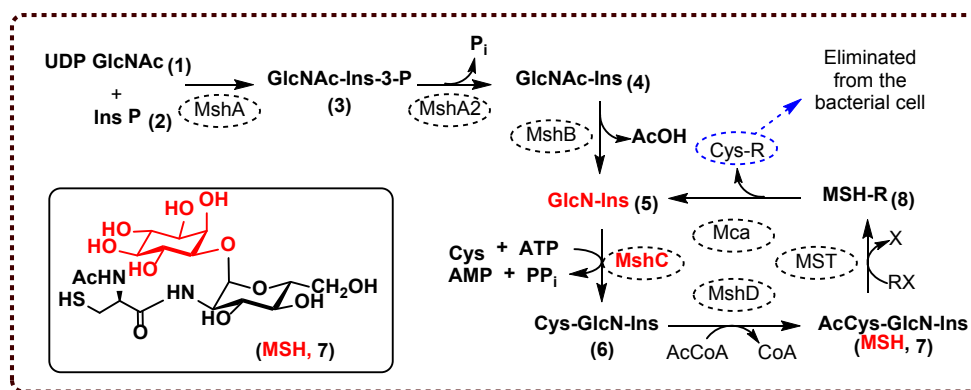
Fig. 1. Mycothiol biosynthesis and metabolic pathway.
