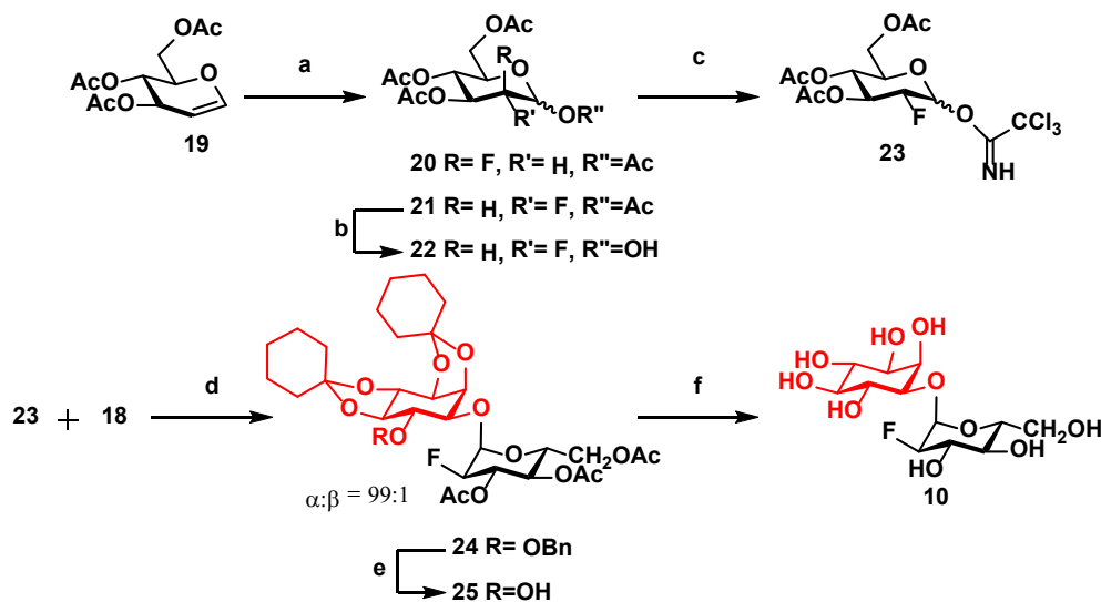
Scheme 2. Reagents and conditions: a) (i) Selectfluor ® , DMF:Water, RT, 12 h, (ii) \text{Ac}_2\text{O} , Pyridine, DMAP, RT, 12 h, ( 20 = 33%, 21 = 58%); b) Ammonium acetate, DMF, RT, 12 h, (96%); c) Trichloroacetonitrile, \text{K}_2\text{CO}_3 , anhydrous DCM, 0 °C, 16 h, (93%); d) TMSOTf, anhydrous DCM, MS-4 Å, -20 °C, 1 h, (78%); e) 10% w/w Pd-C, \text{H}_2 , MeOH, RT, 5 h, (98%); f) (i) \text{NaOMe}/\text{MeOH} , RT, 1 h, (ii) DOWEX 50WX8-100 ion exchange ( \text{H}^+ ) resin, MeOH, 35 °C, 1 h, (98%).
