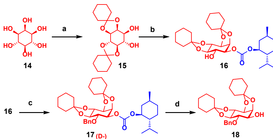
Scheme 1. Reagents and conditions: a) 1,1-dimethoxy cyclohexane, N,N -Dimethylformamide (DMF), p -TsOH, 95–100 °C, 3 h, (23%); b) (i) (\text{Bu}_3\text{Sn})_2\text{O} , toluene (Tol), reflux, 3 h (ii) \text{NaHCO}_3 , (1 R )-(-)-menthyl chloroformate, Tol, 0 °C–RT, 24 h, (73%); c) (i) \text{Ag}_2\text{O} , BnBr, MS-4 Å, anhydrous dichloromethane (DCM), reflux, 6 h, (ii) recrystallization in petroleum ether (45%); d) \text{K}_2\text{CO}_3 , isopropanol:methanol (IPA:MeOH, 1:1), reflux, 6 h, (97%).
