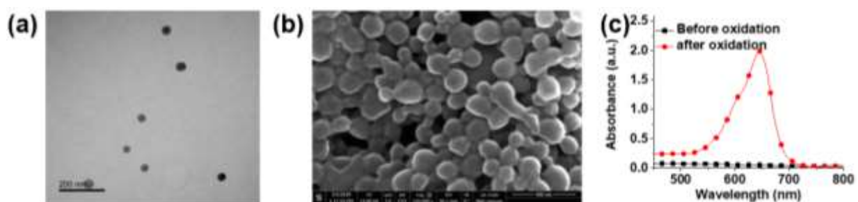
Figure 2. Preparation and characterization of PLGA nanoparticles encapsulating PTX-LMB. (a) TEM micrograph of PTX-LMB-loaded PLGA nanoparticles shows average diameter of 50 nm. (b) SEM micrograph of PTX-MB @ PLGA nanoparticles indicates a diameter of 100-200 nm (scale bar is 400 nm). The difference in size observed between TEM and SEM is due to shrinking of pores in PLGA NPs during TEM (c) Absorbance spectra of the freshly prepared solution of PTX-MB @ PLGA NPs ( 15 \text{ mg mL}^{-1} ) in chloroform (black squares) shows no absorption at 640 nm and the same solution absorbs strongly at 640 nm after oxidation with potassium hexacyanoferrate (III) (red circles). Using the absorbance data from (c), 94.82% of the loaded PTX-MB existed was remained as PTX-LMB.
