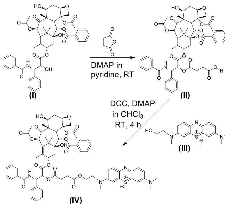
Scheme 1. Design and synthesis of paclitaxel-methylene blue conjugate (PTX-MB). PTX-MB was synthesized through a three step synthesis. The crude product was purified by reverse phase HPLC and isolated as trifluoroacetate salt. The overall isolated yield after HPLC was 13.6%. Inset is a sample of PTX-MB purified by HPLC.
