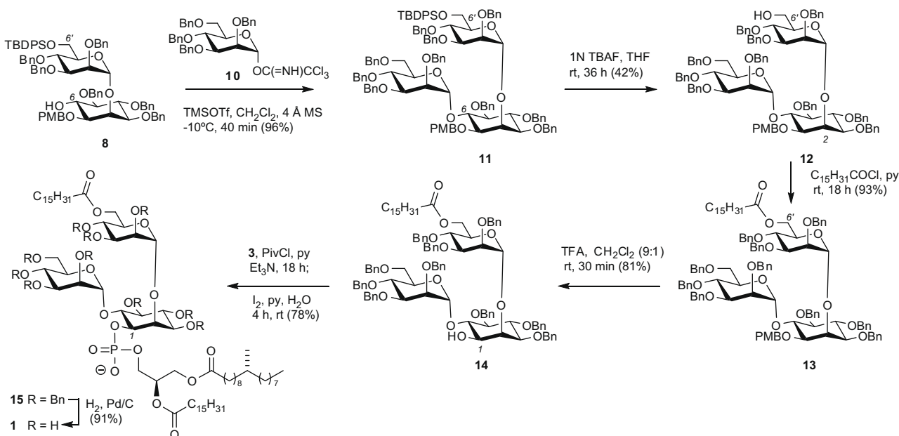
Scheme 3. Assembly of PIM-2 ( 1 ) via [2+1]-glycan construction, lipidation and phosphatidylation.
