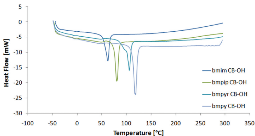
Figure 3. DSC curves of [CB-OH] - -based salts.
