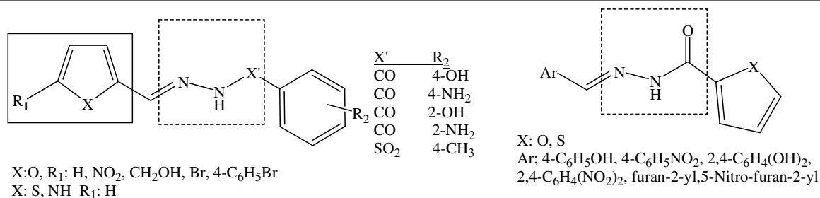
Fig. 2. Molecular modification of nifuroxazide
