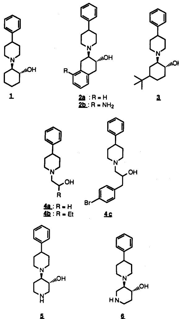
Chart I. Vesamicol Analogs
