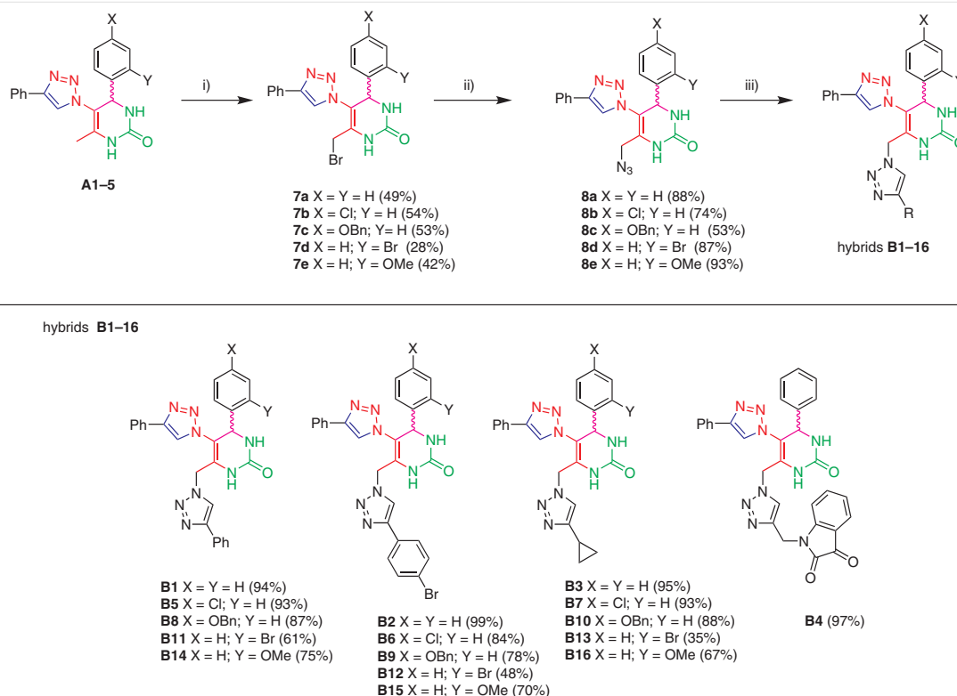
Scheme 3 Synthetic strategy for obtaining the hybrids B1-16 . Reaction conditions: (i) \text{TBABr}_3 (1.5 equiv), dichloromethane, rt, 2 h; (ii) \text{NaN}_3 (1.5 equiv), DMF, 60 °C, microwaves, 30 min; (iii) alkyne (1 equiv), DMF, 90 °C microwaves, 10 min. 15-17
