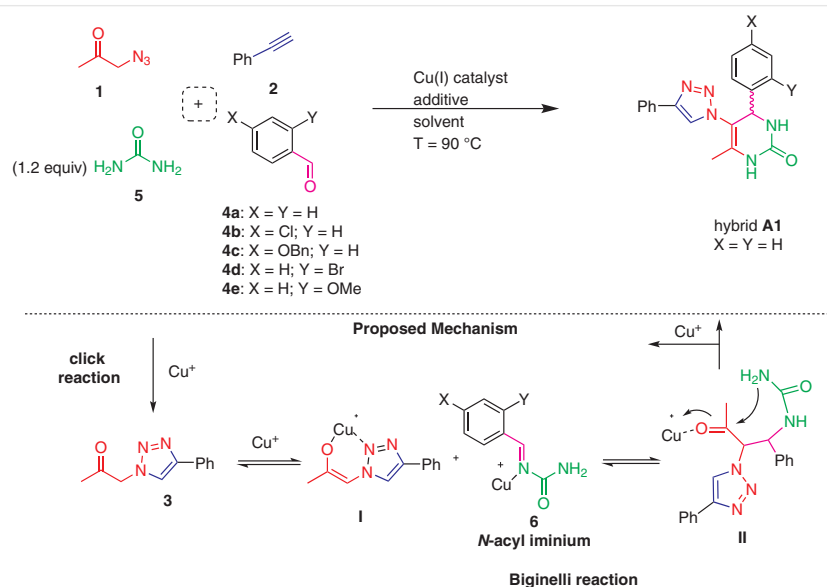
Scheme 2 One-pot synthesis of 1,2,3-triazole-dihydropyrimidinone hybrids A1
