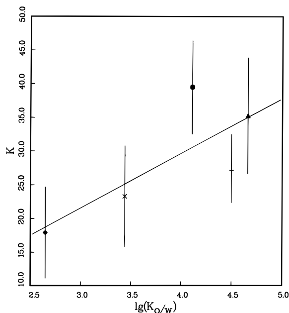
Figure 1. Equilibrium constants for reaction 1 vs the (octanol + water) partition coefficients K_{o/w} of the five solvents used in this study. The solvents and their respective symbols are hexane, ○; heptane, ▲; cyclohexane, ×; 2,2,4-trimethylpentane, +; toluene, ◆.
