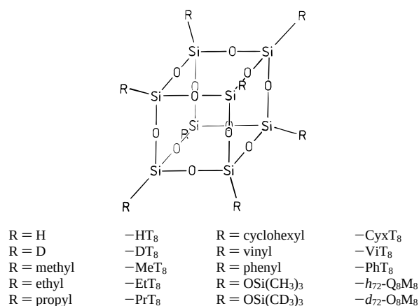
CHART 1. Structures and Denominations of the Substances Used a
