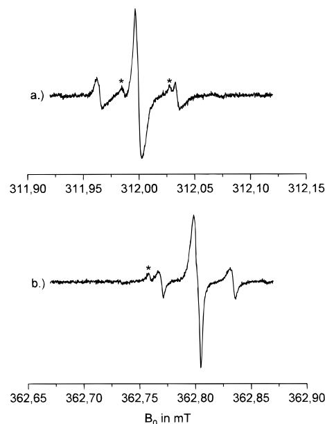
Figure 6. The low- (a) and high-field transitions (b) of hydrogen atoms generated in equimolar mixtures of h_{72} -Q 8 M 8 (a) and d_{72} -Q 8 M 8 , dose: \sim 100 kGy, room temperature. The asymmetry arises from the superposition of spectra of H atoms trapped in either h_{72} -Q 8 M 8 (a) or d_{72} -Q 8 M 8 . The asterisks indicate signals due to H • : [(CD 3 ) 3 SiO] 7 [Si 8 O 12 ]. 21 The doublets arise from the superhyperfinesplitting caused by hydrogen directly attached to silicon (marked by bold H in the formula; a_{\text{H}} \approx 0.0353 mT).
