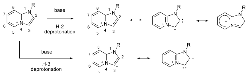
Figure 2. Deprotonation at the 2- vs 3-position.
