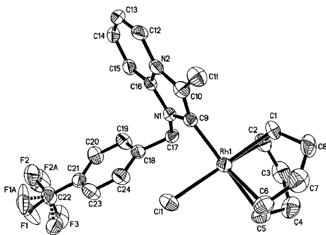
Figure 4. ORTEP diagram of 3d , showing 50% probability ellipsoids.
