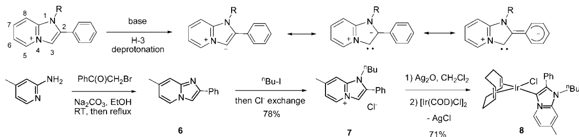
Scheme 2. Metalation at the 3-Position of an Imidazo[1,2- a ]pyridinium
