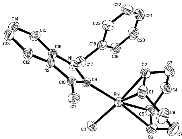
Figure 3. ORTEP diagram of 3a , showing 50% probability ellipsoids.
