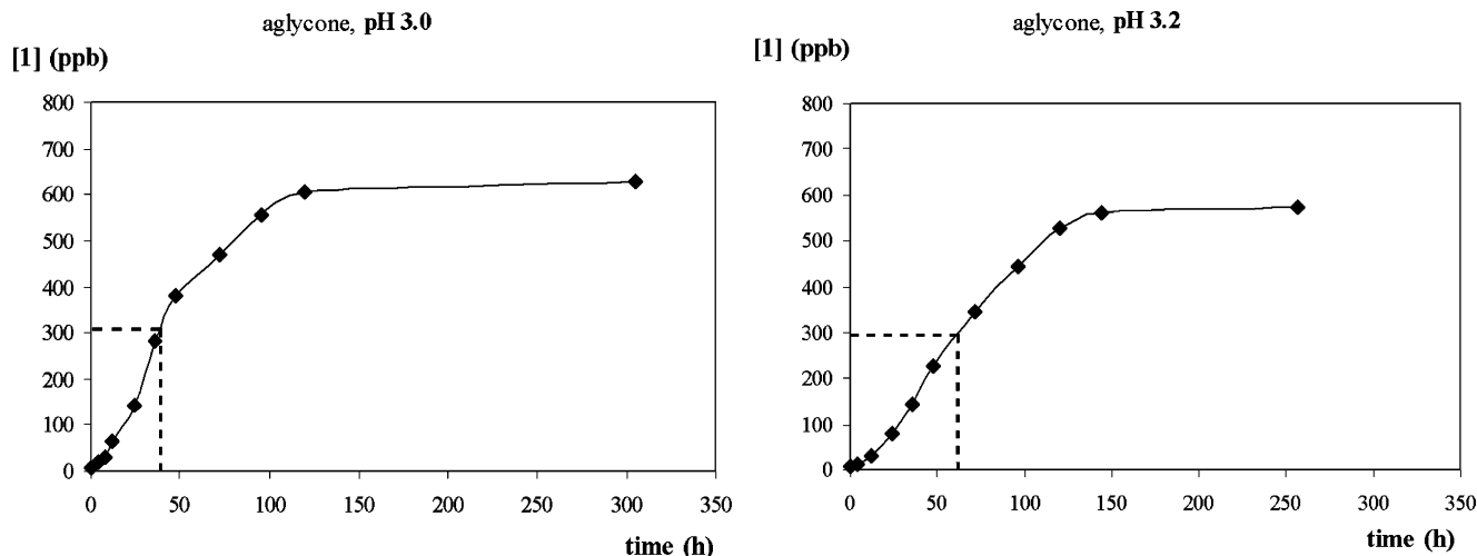
Figure 5. Formation of damascenone ( 1 ) over time during hydrolysis of aglycone 6 at pH 3.0 (left) and pH 3.2 (right). Both hydrolyses were conducted at 25 °C.
