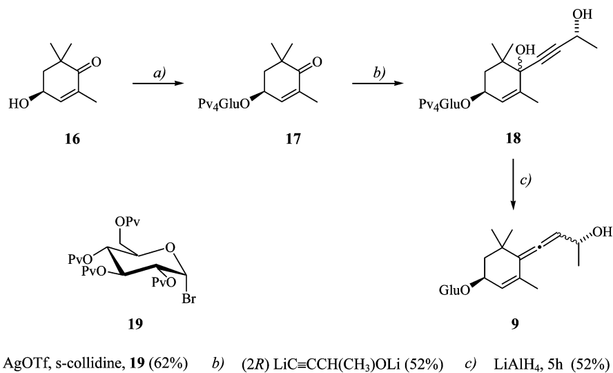
Figure 3. Synthesis of C-3 glycoside 9 .
