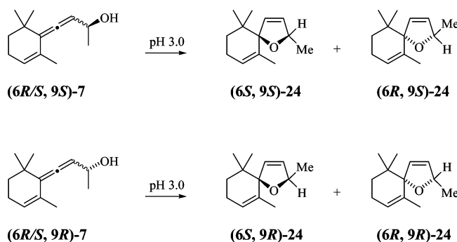
Figure 6. Stereochemical relationship between the starting allenenes 7 and the 7,8-didehydrotheaspirane products obtained.
