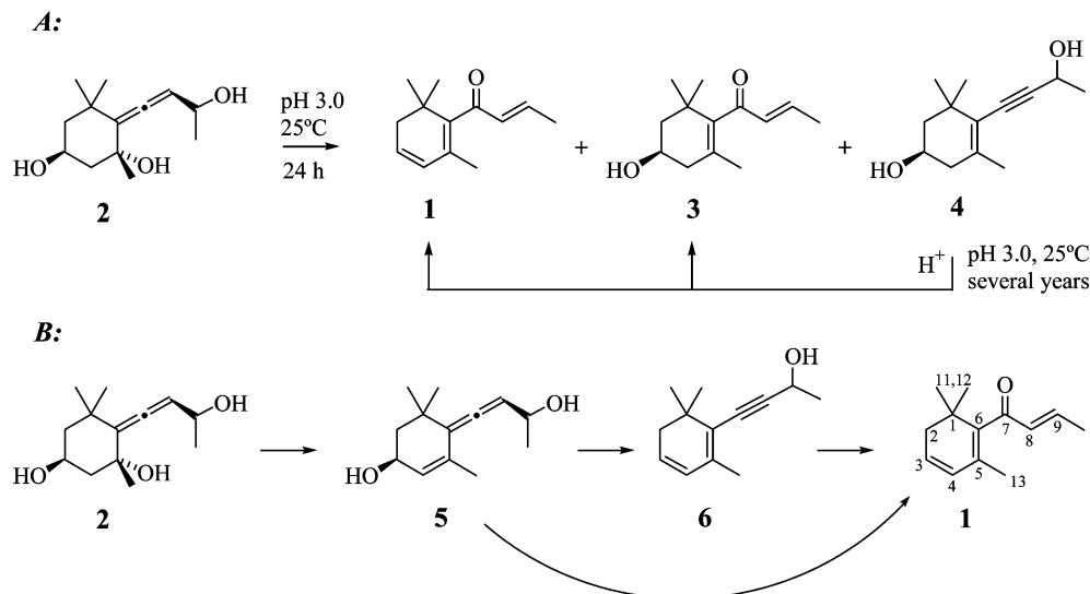
Figure 1. A: Major hydrolysis products of allenic triol 2 . B: Route of formation of damascenone 1 from allenic triol 2 .
