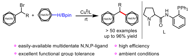
Scheme 1. The design of a general C(sp^3)-C(sp^2) cross-coupling.
