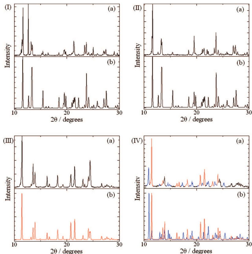
Figure 1. Powder X-ray diffraction patterns of (I) the 1-phenylimidazole- \text{PdCl}_2 complex prepared by method A, (II) the 1-phenylimidazole- \text{PdCl}_2 complex prepared by method B, (III) the 1-phenylimidazole- \text{PdCl}_2 complex prepared by method A, and (IV) the 1-phenylimidazole- \text{PdCl}_2 complex prepared by method B: (a) measured patterns; (b) simulation of powder XRD data using RIETAN-2000. 16
