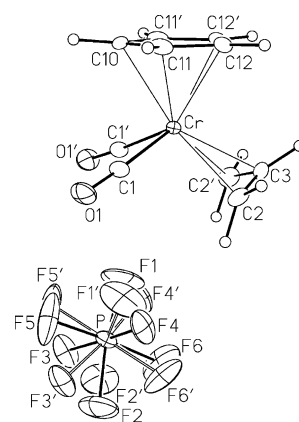
Figure 1. Solid state molecular structure of complex 4 showing the disordered PF 6 - counterion; 0.5 equiv of interstitial DME is omitted. Non-hydrogen atoms are represented by Gaussian ellipsoids at the 20% probability level. Hydrogen atoms are shown with arbitrarily small thermal parameters. See Table 2 for selected bond lengths and angles of the cation. Complete listings of bond lengths and angles are available as Supporting Information.
