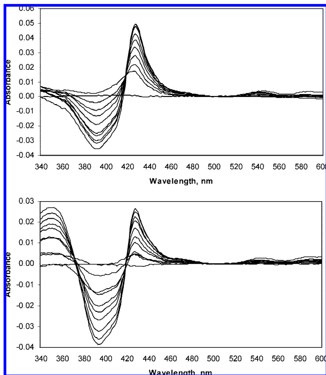
Figure 3. Difference spectra for the binding of 44a (top panel) and 44d (bottom panel) to recombinant T. cruzi L14DM. Compounds were added to 2.2 \mu M enzyme in increments of 0.2 \mu M. Maximum difference spectra were obtained with equimolar enzyme and compound. The absorbance around 360 nm in the spectra with 44d is attributed to the compound alone. Binding of compound to enzyme caused an increase in absorbance at \sim 440 nm and a decrease at \sim 390 nm.
