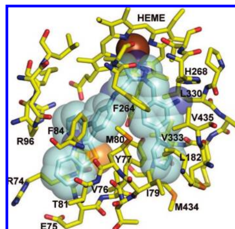
Figure 2. Homology model of T. cruzi L14DM in complex with 44d .
