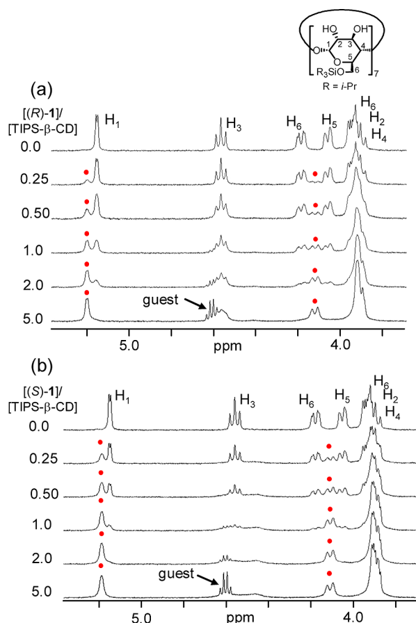
Figure 1. ^1\text{H} NMR spectral changes observed for TIPS- \beta -CD ( 1.0 \times 10^{-3} M) upon addition of (a) (R)-1 and (b) (S)-1 in benzene- d_6 at 25 ^\circ\text{C} . Red circles denote new signals that appeared upon addition of 1.
