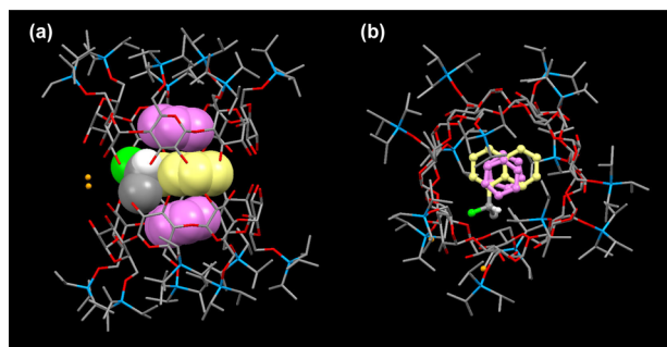
Figure 2. Crystal structure of the supramolecular TIPS- \beta -CD capsule-( S )-1 inclusion complex. (a) Side view. TIPS- \beta -CD is shown with a cylinder representation, whereas ( S )-1 and benzene are shown with space-filling representations. The O atoms in H 2 O are shown as orange balls. H atoms except for the \alpha -methine hydrogen of ( S )-1 have been omitted for clarity. (b) Top view. TIPS- \beta -CD is shown with a cylinder representation, whereas ( S )-1 and benzene are shown with ball-and-stick representations. O atoms in H 2 O are shown as orange balls. Color labels: gray, carbon in TIPS- \beta -CD and aliphatic carbon in ( S )-1; cyan, silicon; red, oxygen in TIPS- \beta -CD; yellow, naphthalene ring; violet, benzene molecule; orange, oxygen in H 2 O.
