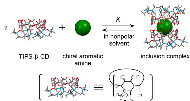
Scheme 1. Formation of an Inclusion Complex between a Supramolecular TIPS- \beta -CD Nanocapsule and a Chiral Aromatic Amine in a Nonpolar Solvent
