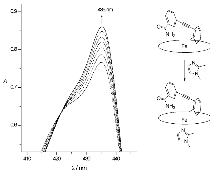
Fig. 4. Formation of the five-coordinate complex 6 \cdot \text{Fe}(\text{DiMeIm}) upon addition of DiMeIm to 6 \cdot \text{Fe} , as monitored by the increase in intensity of the Soret band at 435 nm. Spectra were recorded in intervals of 15 min.
