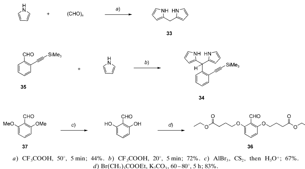
Scheme 7. Preparation of Precursors for the Macrocyclization to Porphyrin 32·2H
