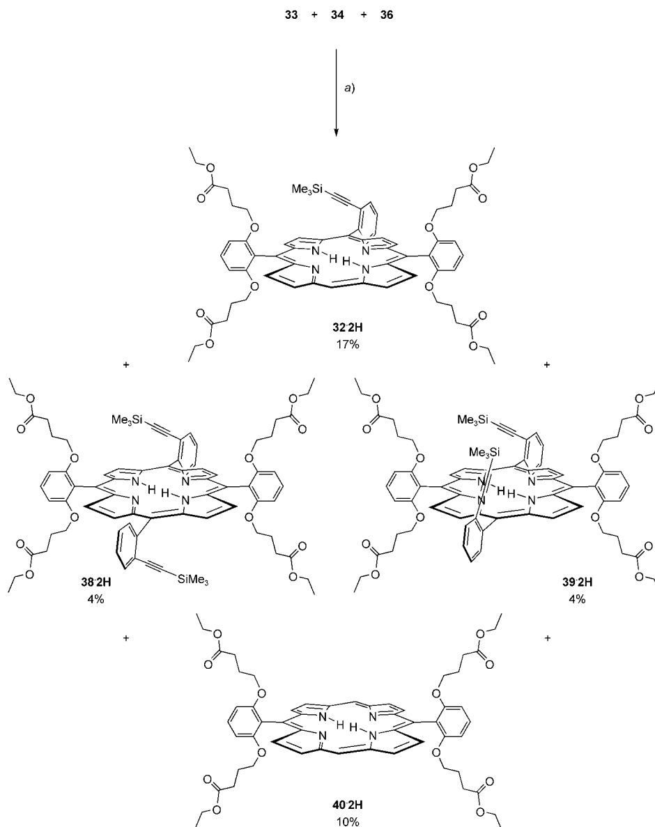
Scheme 8. Synthesis of Porphyrin 32·2H
