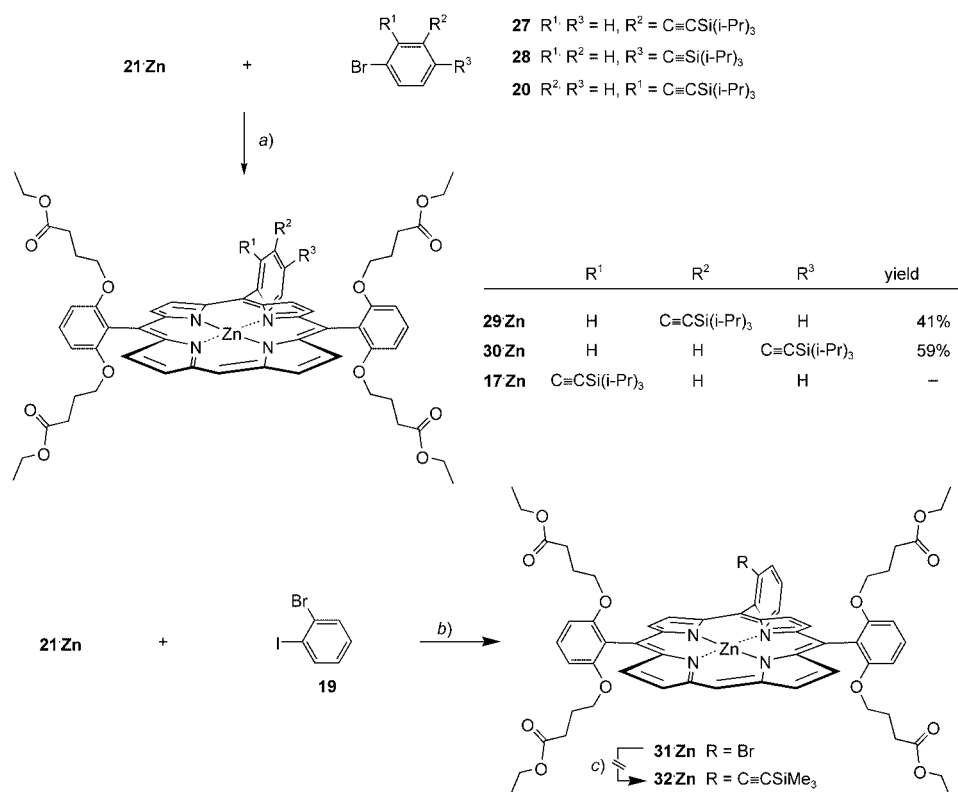
Scheme 6. Experiments Demonstrating the Difficulty to Introduce an ortho-Ethynylated meso-Aryl Ring in Cross-Coupling Reactions with Porphyrin Boronate 21·Zn
