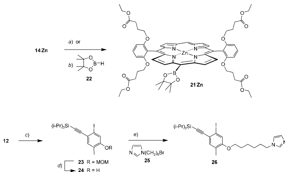
Scheme 4. Synthesis of Precursors for Suzuki Cross-Couplings Using Porphyrinylboronates as Transmetallating Agents
