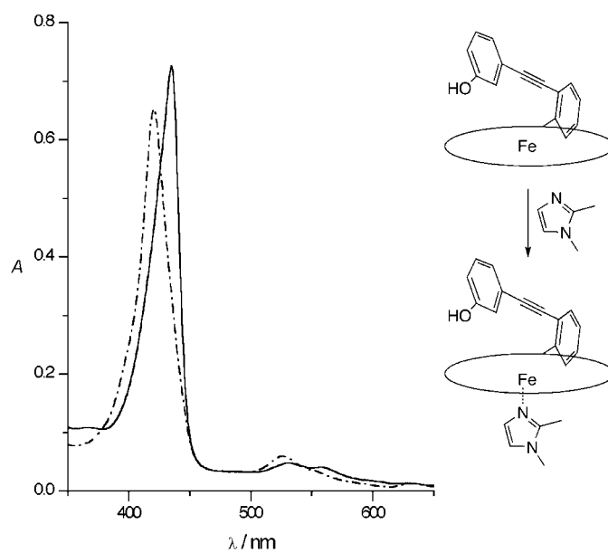
Fig. 3. Upon addition of DiMeIm, the maximum of the Soret band of 4 \cdot \text{Fe} (420 nm, - - - -) shifts to 435 nm (—), indicative of formation of the five-coordinate complex 4 \cdot \text{Fe}(\text{DiMeIm}) . DiMeIm = 1,2-Dimethyl-1H-imidazole.
