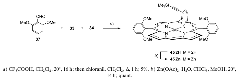
Scheme 10. Synthesis of \text{Zn}^{\text{II}} Porphyrin 45·Zn
