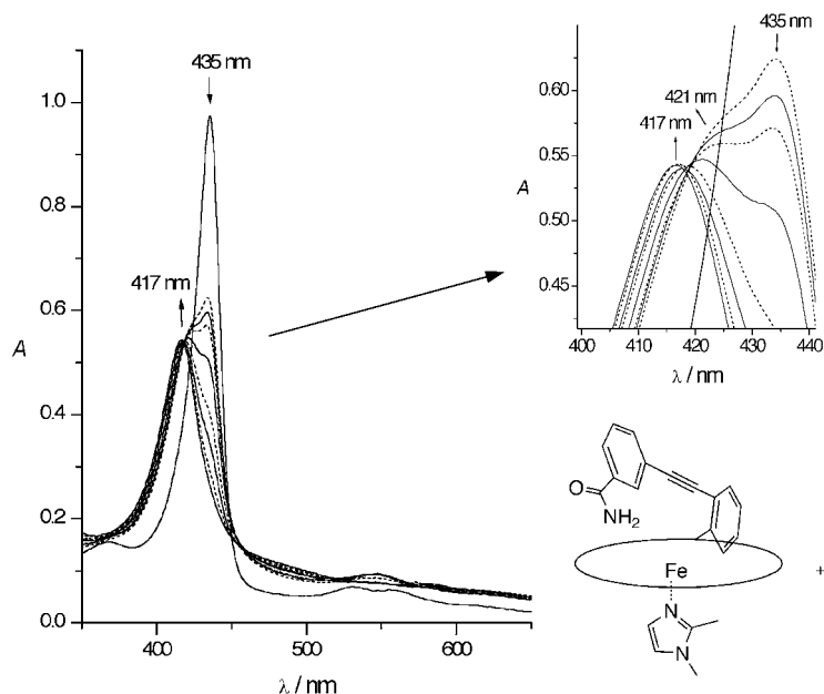
Fig. 7. Upon addition of O_2 to 1 \cdot Fe(DiMeIm) , the Soret band shifts from 435 to 417 nm. In the course of the irreversible oxidation, a shoulder is observed at 421 nm, which could be indicative of the intermediate Fe(II)-O_2 complex.
