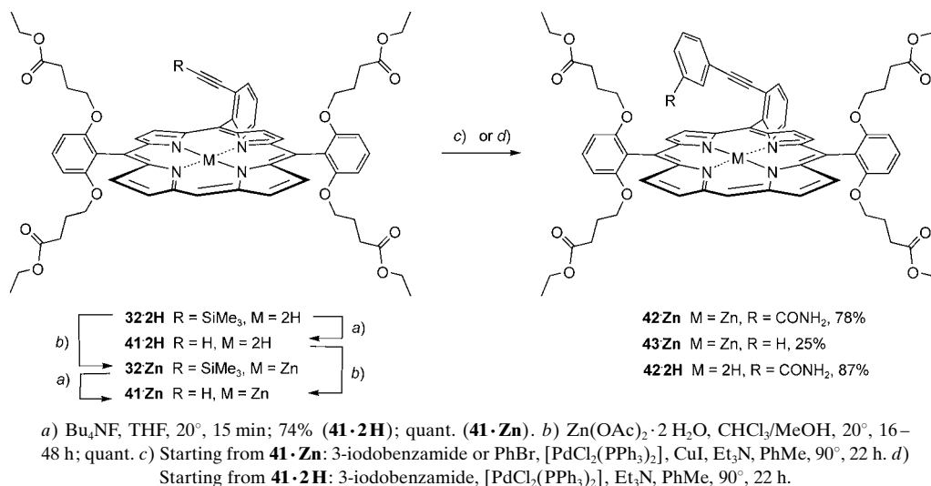
Scheme 10. Synthesis of \text{Zn}^{\text{II}} Porphyrin 45·Zn
