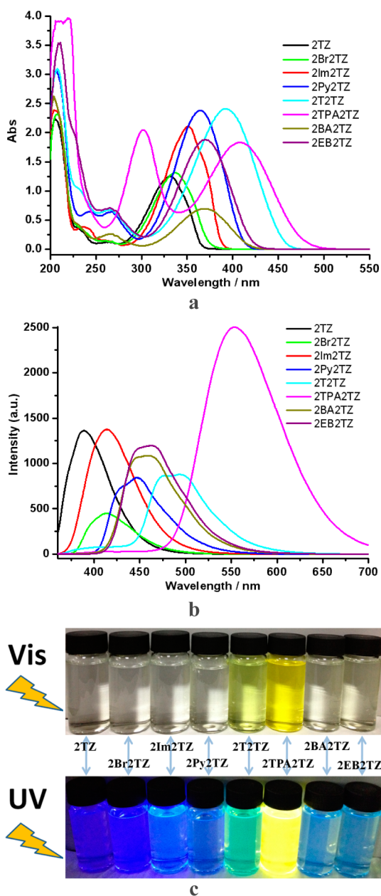
Figure 1. UV-vis absorption spectra (a), fluorescence emission spectra excited at 350 nm (b), and their visual photographs (c) for the heterocyclic aromatic compounds in their methanol solutions at room temperature with the same concentration of 5.0 \times 10^{-5} \text{ mol}\cdot\text{L}^{-1} .
