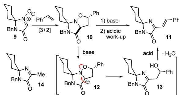
Scheme 1. Formation of 11
