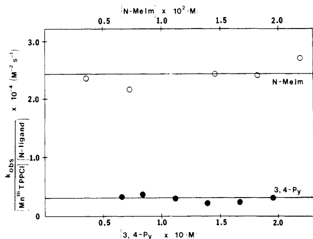
Figure 6. Plots of k_{\text{obsd}}/[(\text{TPP})\text{Mn}^{\text{III}}\text{Cl}][\text{N-ligand}] vs. [\text{3,4-Py}] (●) and [\text{N-MeIm}] (○) for the oxygen transfer from \text{Ph}_2\text{C}(\text{CN})\text{OOH} to (\text{TPP})\text{Mn}^{\text{III}}\text{Cl} with 3,4-lutidine and N -methylimidazole as the N-ligand.
