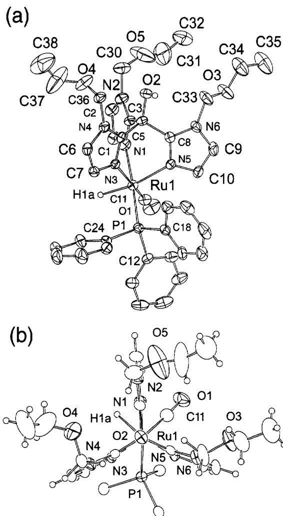
Fig. 3. ORTEP of [\{Ru((emim)_3COH)(PPh_3)(CO)H\}^+ Cl^-] ( 3b ); 20% thermal ellipsoids are shown for the non-hydrogen atoms; hydrogen atoms have an arbitrary radius of 0.1 Å. (a) Numbering scheme; (b) view of 3b down the axis through the central carbon of the (emim)_3COH ligand and the ruthenium atom.
