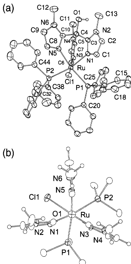
Fig. 2. ORTEP of [\{RuCl(PPh_3)_2((mim)_3COH)\}^+ Cl^-] ( 2 ); 30% thermal ellipsoids are shown for the non-hydrogen atoms; hydrogen atoms have an arbitrary radius of 0.1 Å. (a) Numbering scheme; (b) view of 2 down the axis through the central carbon of the (mim)_3COH ligand and the ruthenium atom.
