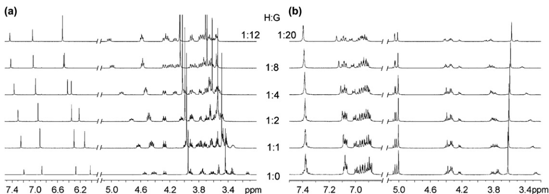
Figure 6. 1 H NMR titration spectra of (a) BC5 with CsPF 6 in acetone- d 6 and (b) m-TBBC6 with CsPF 6 in CDCl 3 –CD 3 CN (1:3) showing the changes in the aromatic and crown ether area of the spectra with different host–guest ratios.
