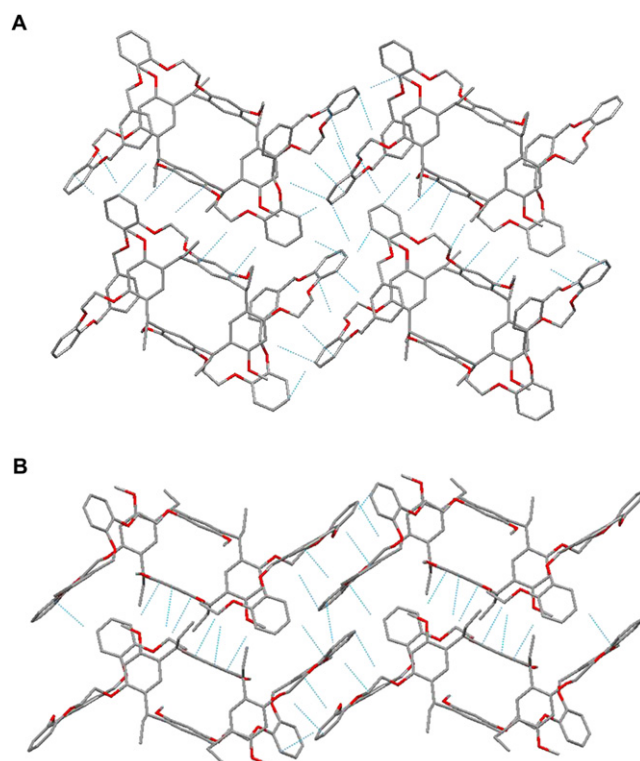
Figure 5. Crystal packing of the structures A (top) and B (bottom) of m -TBBC6 (top views). Blue lines indicate the CH– \pi and \pi – \pi interactions between the neighboring molecules. Hydrogens and solvent molecules are omitted for clarity.
