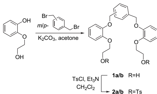
Scheme 2. Synthesis of aromatic crown bridges of m/p-TBBC6 .
