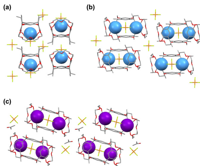
Figure 8. Crystal packing of the complexes of BC5 with \text{CsPF}_6 and \text{RbPF}_6 : (a) sideview of BC5 · \text{CsPF}_6 (same for the complex of BC5 · \text{RbPF}_6 ), (b) top view of BC5 · \text{CsPF}_6 , and (c) top view of BC5 · \text{RbPF}_6 . Hydrogens are omitted for clarity.
