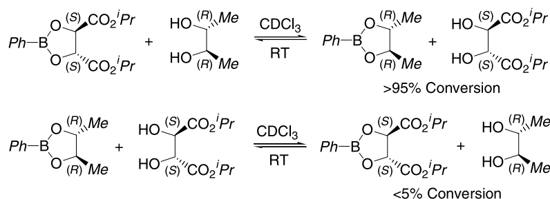
Fig. 5. Transesterification of boronic ester 1
