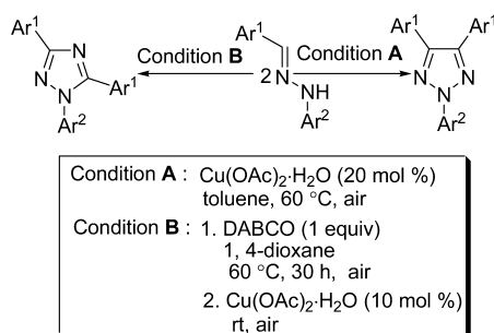
Scheme 1. Cu(II)-Catalyzed C–H Functionalization of Bisarylhydrazones
