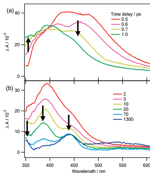
Figure 1. Transient UV–vis spectra produced upon 310 nm photolysis of \text{PhCH}=\text{CHCN}_2\text{CO}_2\text{CH}_3 in acetonitrile.
