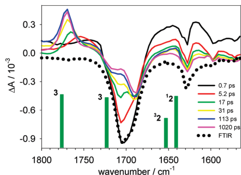
Figure 2. Transient IR spectra produced upon 270 nm photolysis of \text{PhCH=CHCN}_2\text{CO}_2\text{CH}_3 in chloroform. The dotted curve is the FTIR spectrum of \text{PhCH=CHCN}_2\text{CO}_2\text{CH}_3 in chloroform. Bars represent the calculated frequencies for singlet carbene ( ^1\mathbf{2} ), triplet carbene ( ^3\mathbf{2} ), and cyclopropene ( \mathbf{3} ).
