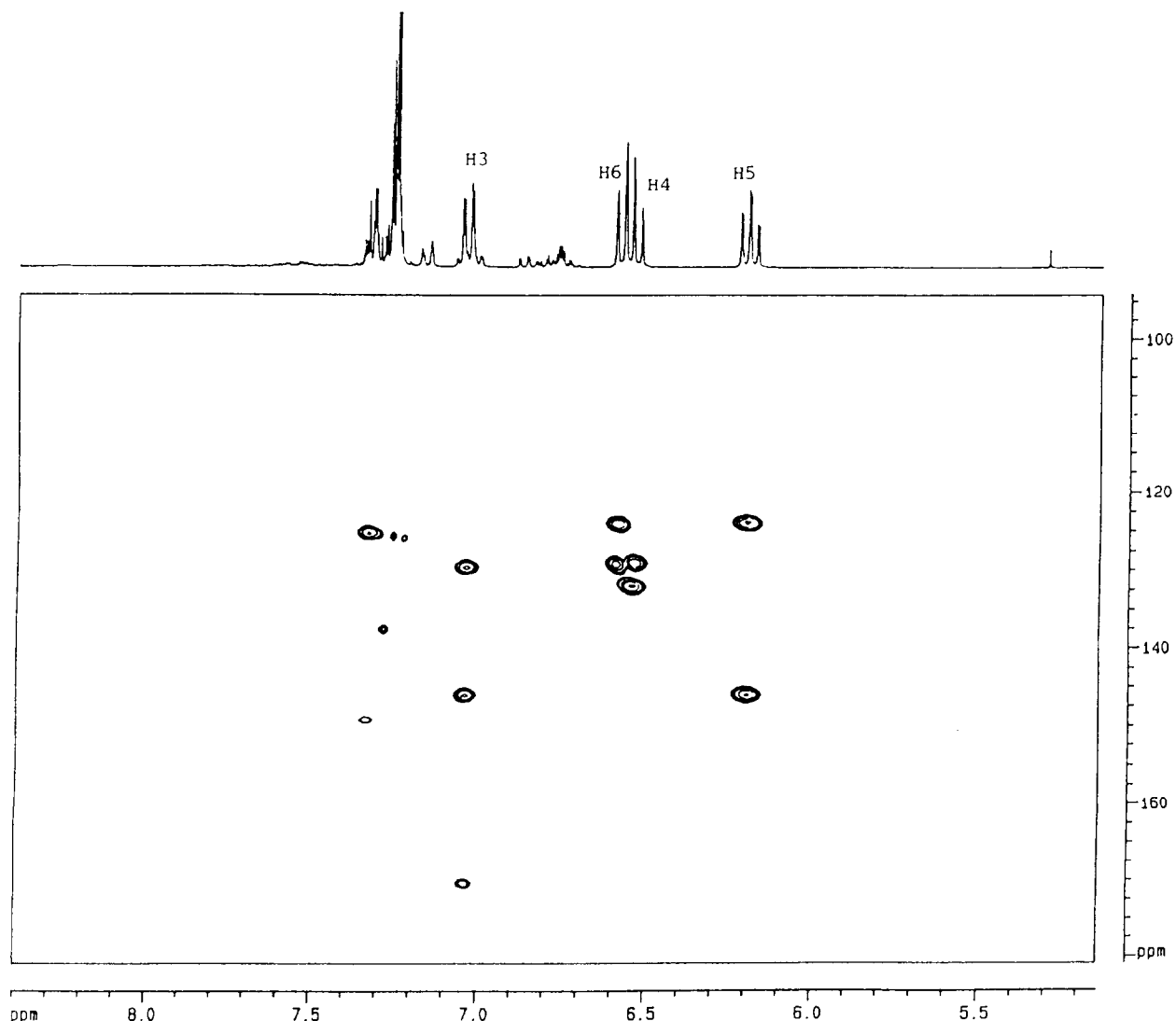
Fig. 2. HMBC experiment for 1c .
