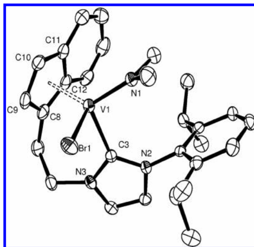
Figure 3. ORTEP representation of complex (Ind-NHC)V(NMe 2 )-Br showing 50% probability ellipsoids. H atoms are omitted for clarity. Selected bond lengths (Å) and angles (deg) with estimated standard deviations: V(1)–N(1) 1.885(3); V(1)–C(3) 2.185(3); N(3)–C(3) 1.363(4); N(2)–C(3) 1.388(4); N(3)–C(3)–N(2) 103.5(3); N(2)–C(3)–V(1) 132.0(2); N(3)–C(3)–N(2) 103.5(3).
