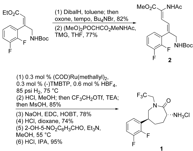
Scheme 2. Synthesis of Caprolactam 1
