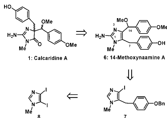
Figure 2. Retrosynthetic analysis of calcaridine A.
