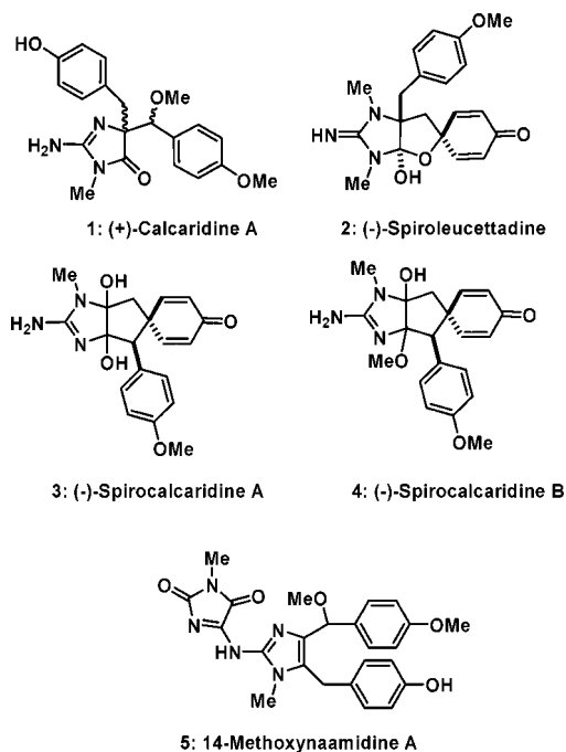
Figure 1. Selected Leucetta alkaloids.
