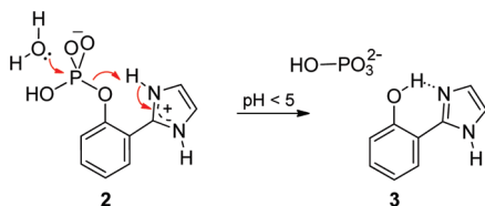
Scheme 2. Mechanism of Intramolecular General Acid Catalysis of the Hydrolysis of Phosphate Monoester 2 6
