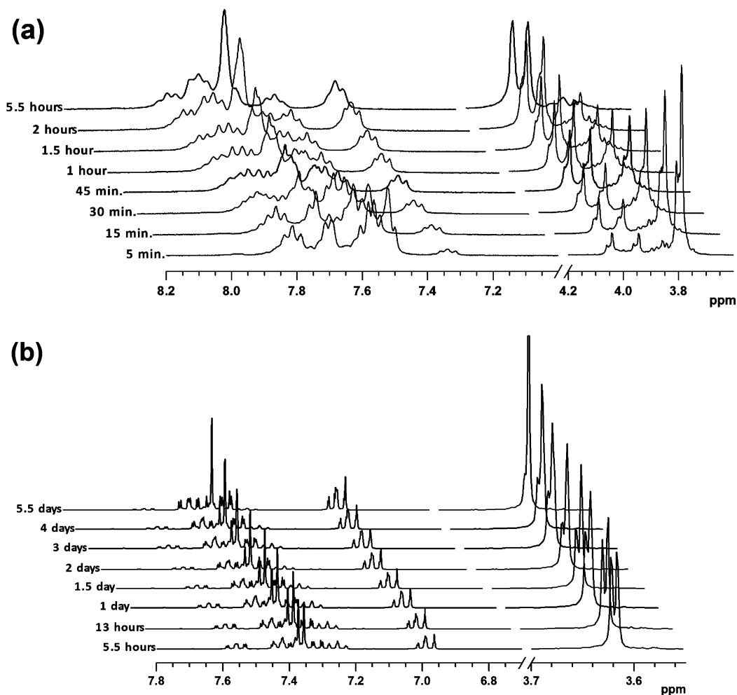
Figure 10. Progressive 1 H NMR spectra of the hydrolysis reaction of BMIPP . (a) Hydrolysis of BMIPP at pD 7.2 and (b) hydrolysis of the intermediate monoester Me-2 at pD 1.5, in D 2 O, at 60 °C. Signals are identified in Table 6.
