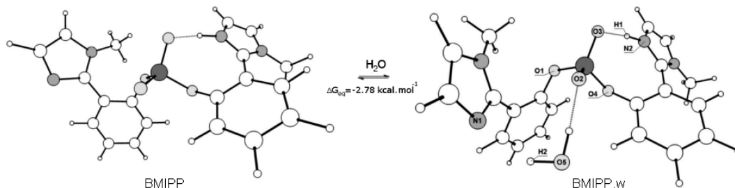
Figure 3. B3LYP gas phase optimized structures of BMIPP ^\pm and BMIPP ^\pm\cdot\text{w} showing the \Delta G_{\text{eq}} involved in the organic phosphate–water complex formation. The basis set used is given in the Experimental Section.
