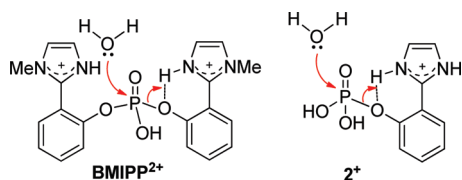
Scheme 5. Suggested Mechanism for the Hydrolysis of BMIPP 2+ in Strong Acid, Compared with the Similar Reaction of 2 6 (See the Text)
