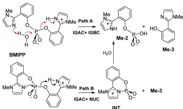
Scheme 3. Alternative Mechanisms for the Rapid Hydrolysis of the Phosphodiester BMIPP , Involving Intramolecular General Acid Catalysis (IGAC) by the Imidazolium Group of General Base (Path A) or Nucleophilic Catalysis (Path B) by the Imidazole Free Base
