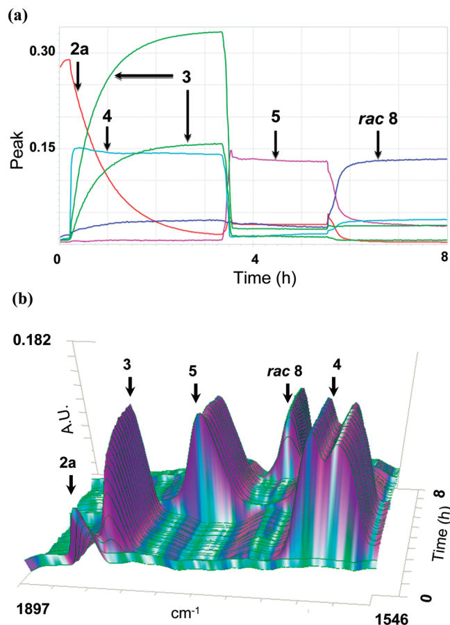
Figure 1. (a) Trends recorded for the reaction of triphosgene (2a) to phosgene (3), the reaction of phosgene (3) with intermediate 4, and the reaction of carbonyl chloride 5 with piperazine 6 over time (h). (b) Surface plot for the reactions.
