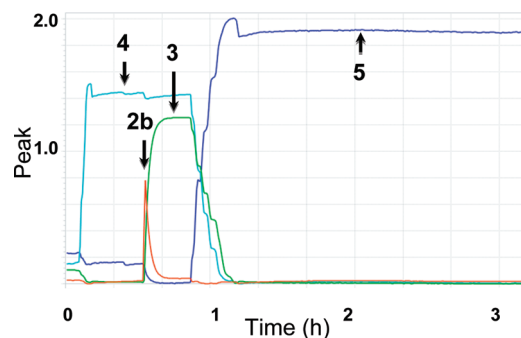
Figure 2. Trends recorded over time (h) for the reaction of diphosgene (2b) to phosgene (3), followed by the reaction of phosgene (3) with intermediate 4 upon addition of DIPEA.
