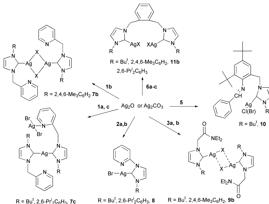
Scheme 2 The synthesis of silver complexes. See Experimental section for details. Compounds in bold have been structurally characterised.
