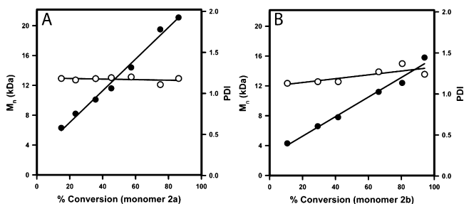
Figure 9. M_n (●) and PDI (○) vs conversion for the \text{Ni}(\text{dppe})\text{Cl}_2 -catalyzed polymerizations of (A) 2a and (B) 2b in THF at 0^\circ\text{C} ( [\text{2a}] = 0.10\text{ M} ; [\text{2b}] = 0.20\text{ M} ; [\text{Ni}(\text{dppe})\text{Cl}_2] = 0.0015\text{ M} ).
