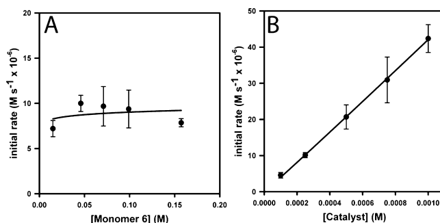
Figure 3. (A) Plot of initial rate vs [monomer] for the polymerization of 6 in THF at 0 °C ([Ni(dppe)Cl 2 ] = 0.00025 M). The curve depicts an unweighted least-squares fit to the expression initial rate = a[\text{monomer}]^n that gave a = 10 \pm 3 and n = 0.05 \pm 0.09 . (B) Plot of initial rate vs [catalyst] for the polymerization of 6 in THF at 0 °C ([ 6 ] = 0.10 M). The curve depicts an unweighted least-squares fit to the expression initial rate = a[\text{catalyst}]^n that gave a = (4.9 \pm 0.8) \times 10^4 and n = 1.02 \pm 0.02 .
