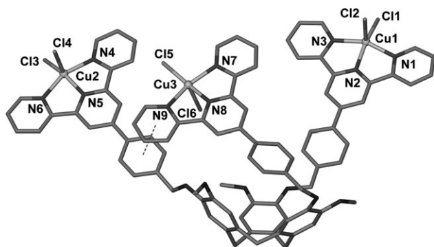
Figure 1. Trinuclear [\text{Cu}_3\text{Cl}_6(\mathbf{1})] species from the crystal structure of [\text{Cu}_3\text{Cl}_6(\mathbf{1})]\cdot\text{CH}_3\text{CN}\cdot 1.5\text{H}_2\text{O} . Intramolecular \pi - \pi stacking interaction is shown as dashed line. Selected bond lengths [Å] and angles [°]: Cu1–N1 2.062(8), Cu1–N2 1.955(7), Cu1–N3 2.049(8), Cu1–Cl1 2.250(2); Cu1–Cl2 2.434(3), Cu2–N4 2.039(9), Cu2–N5 1.942(7), Cu2–N6 2.052(9), Cu2–Cl3 2.254(3), Cu2–Cl4 2.415(9), Cu3–N7 2.075(10), Cu3–N8 1.922(10), Cu3–N9 2.077(9), Cu3–Cl5 2.206(4), Cu3–Cl6 2.647(4); N2–Cu1–Cl1 154.9(2), N1–Cu1–Cl1 99.5(2), N3–Cu1–Cl1 98.7(2), N2–Cu1–Cl2 99.3(2), N3–Cu1–Cl2 96.7(2), N1–Cu1–Cl2 93.3(2), Cl1–Cu1–Cl2 105.80(10), N5–Cu2–Cl3 153.3(2), N4–Cu2–Cl3 98.4(2), N6–Cu2–Cl3 98.8(3), N5–Cu2–Cl4 99.6(2), N4–Cu2–Cl4 96.9(3), N6–Cu2–Cl4 92.4(3), Cl3–Cu2–Cl4 107.07(12), N8–Cu3–Cl5 172.2(3), N7–Cu3–Cl5 100.3(4), N9–Cu3–Cl5 99.0(3), N8–Cu3–Cl6 85.7(3), N7–Cu3–Cl6 89.9(3), N9–Cu3–Cl6 99.2(2), Cl5–Cu3–Cl6 102.15(16).
