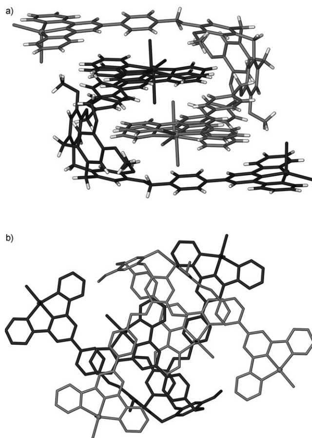
Figure 2. Two views of the homomeric hand-shake dimer of complex [\text{Cu}_3\text{Cl}_6(\mathbf{1})] from the crystal structure of [\text{Cu}_3\text{Cl}_6(\mathbf{1})]\cdot\text{CH}_3\text{CN}\cdot 1.5\text{H}_2\text{O} .
