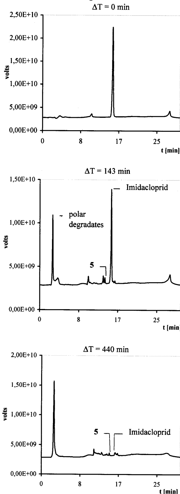
Figure 4. HPLC chromatograms of imidacloprid.
