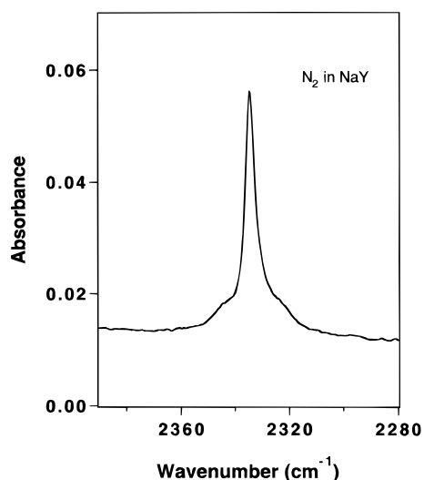
Figure 5. Induced infrared fundamental absorption of N 2 loaded into zeolite NaY at -78^{\circ}\text{C} . The loading level corresponds to 1.3 molecules per supercage.
