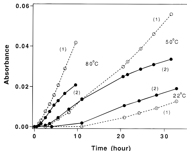
Figure 4. Absorbance growth kinetics of the 1705-cm -1 cyclohexanone band (curve 1) and the 1367-cm -1 cyclohexyl hydroperoxide absorption (curve 2) upon thermal reaction at 22, 50, and 80 °C. The size of the circles indicates the peak-to-peak noise.
