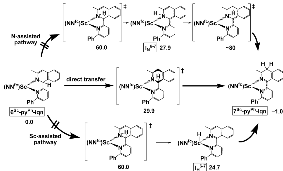
Figure 2. Pathways studied computationally for the isomerization of 6^{\text{Sc-py}^{\text{Ph}}\text{-iqn}} to 7^{\text{Sc-py}^{\text{Ph}}\text{-iqn}} ; all energies given in kcal/mol.
