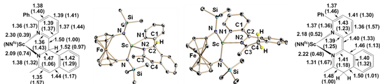
Figure 1. Extreme left and right: Relevant metrical parameters (in Å) from the X-ray crystal structures of 6^{\text{Sc-py}^{\text{Ph-iqu}} and 7^{\text{Sc-py}^{\text{Ph-iqu}} and, in parentheses, bond orders calculated by ADF2008.01 from geometry optimizations on the full molecules. Center: ORTEP representations of 6^{\text{Sc-py}^{\text{Ph-iqu}} and 7^{\text{Sc-py}^{\text{Ph-iqu}} with ellipsoids drawn at 50% probability ('Bu methyl, pyridine phenyl groups, and irrelevant hydrogen atoms were removed for clarity).
