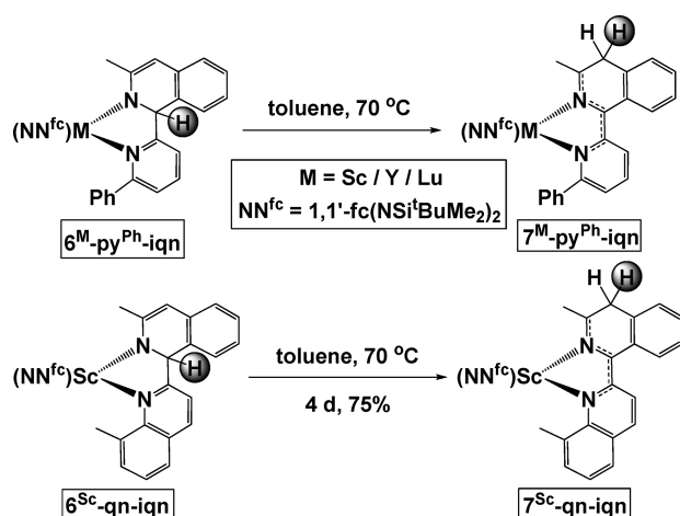
Scheme 3. Isomerization of Biheterocyclic Ligands in 6^{\text{M}} Complexes (M = Sc, Y, Lu)
