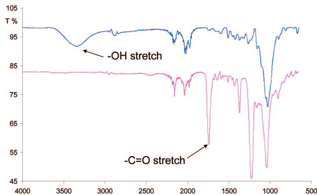
Figure 4. IR spectra (ATR) of vacuum-dried (50 °C) spruce wood sawdust (top spectrum) and acetylated sample regenerated from [amim]Cl (bottom spectrum; entry 3b, Table 1 ). The signals for the \text{—OH} and \text{—C=O} stretching bands are indicated.
