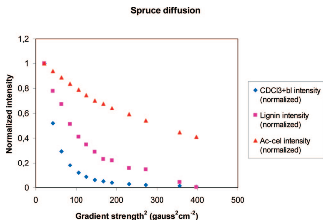
Figure 6. Diffusion measurements on acetylated Norway spruce sample dissolved in \text{CDCl}_3 ; diffusion rates of \text{CDCl}_3 (◆), lignin \beta -O-4 \alpha proton (■), and cellulose H-1 (▲).
