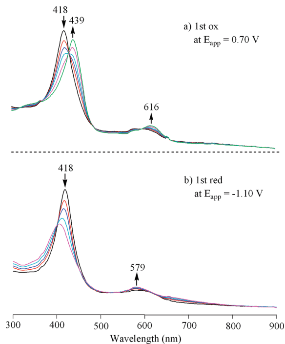
Figure 10. UV–visible spectral changes of \text{Co}^{\text{II}} azahemiporphycene 15 during (a) the first oxidation at 0.70 V and (b) the first reduction at -1.10 V in PhCN, 0.1 M TBAP.
