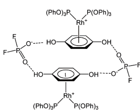
Figure 5. Dimeric structure of 1^+\text{OPf}^- (compare to 1^+\text{OTf}^- in Figure 4).
