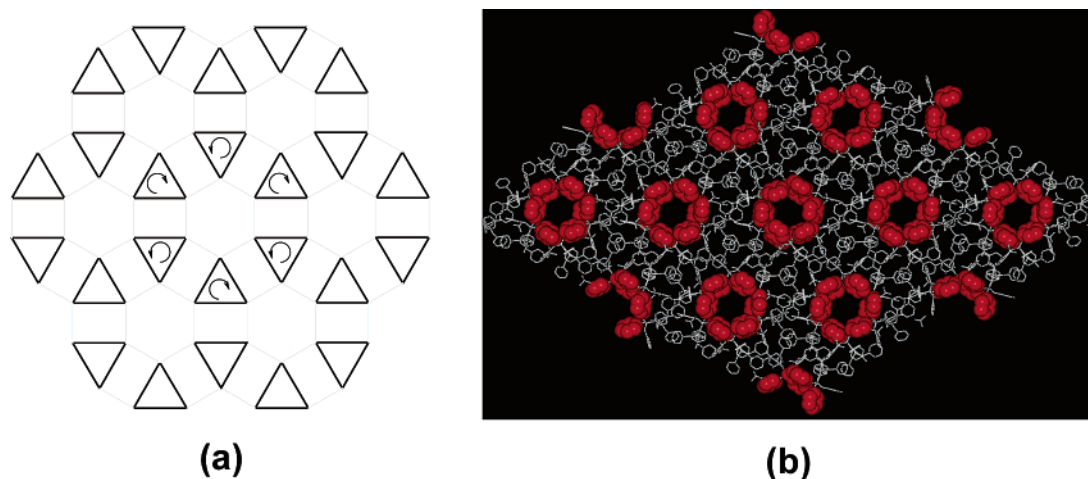
Figure 10. (a) 3-D packing of the C_3 helices in 1^+\text{ClO}_4^- and 1^+\text{BF}_4^- . (b) Depiction of the resultant hydrophobic channels (red).
