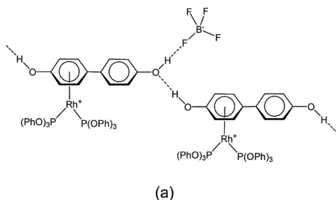
Figure 7. (a) 1-D hydrogen-bonded chain structure in 3^+\text{BF}_4^- . (b) Structure of 3^+\text{BF}_4^- with disordered solvent (violet) in channels that are lined with phenyl rings.
