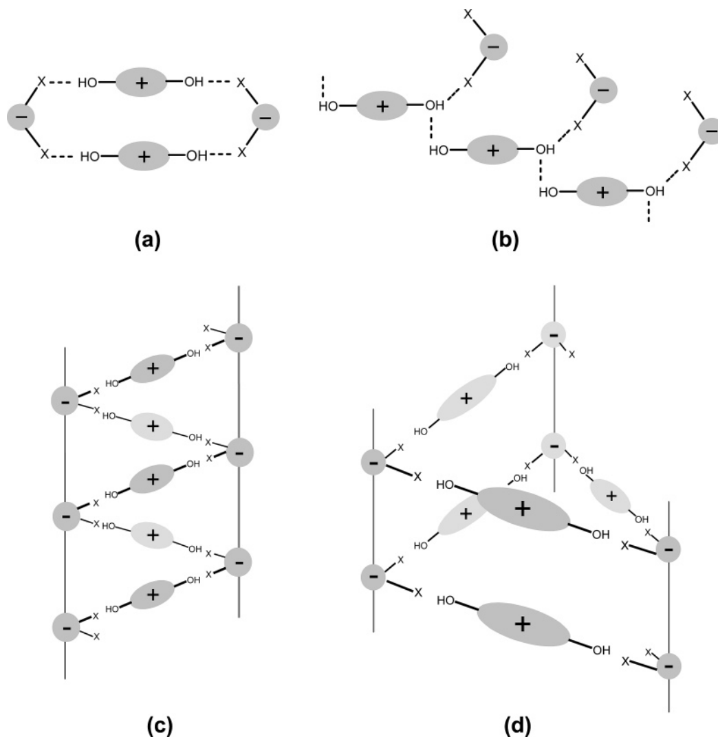
Figure 1. Hydrogen-bonded structural patterns found in the solid state for [1^+-3^+]\text{X}^- : (a) dimeric; (b) 1-D chain; (c) \text{C}_2 helical; (d) \text{C}_3 helical.
