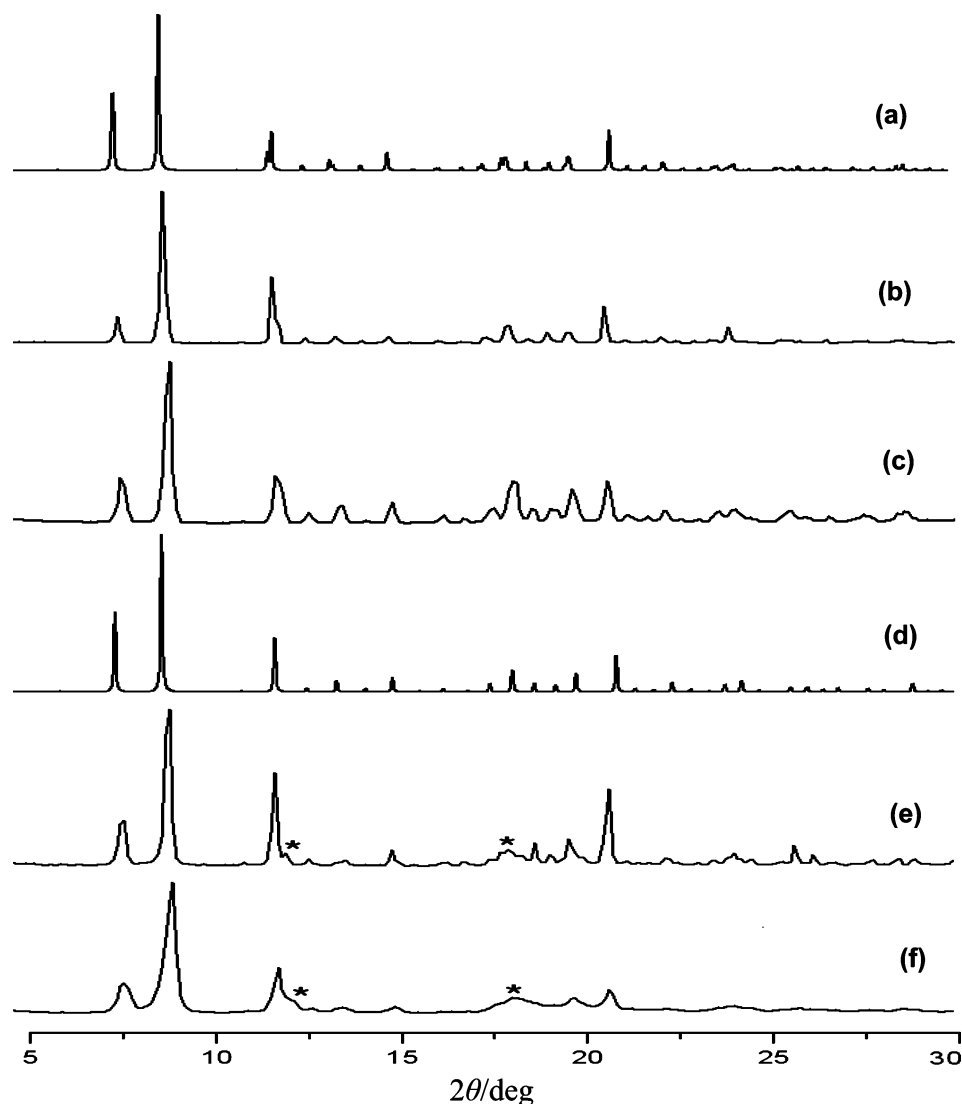
Figure 11. PXRD patterns: (a) simulated pattern of 1^+\text{ClO}_4^- from single-crystal X-ray data; (b) experimental pattern of macrocrystals of 1^+\text{ClO}_4^- ; (c) experimental pattern of microcrystals formed by simple precipitation of 1^+\text{ClO}_4^- ; (d) simulated pattern of 1^+\text{BF}_4^- from single-crystal X-ray data; (e) experimental pattern of macrocrystals of 1^+\text{BF}_4^- ; (f) experimental pattern of microcrystals formed by simple precipitation of 1^+\text{BF}_4^- .
