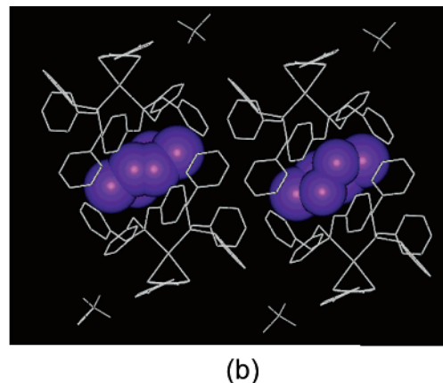
Figure 7. (a) 1-D hydrogen-bonded chain structure in 3^+\text{BF}_4^- . (b) Structure of 3^+\text{BF}_4^- with disordered solvent (violet) in channels that are lined with phenyl rings.
