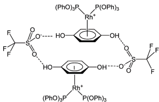
Figure 4. Dimeric structure of 1^+\text{OTf}^- , which features charge-assisted hydrogen-bonding and \pi - \pi -stacking interactions.
