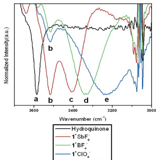
Figure 14. IR spectra in the \nu_{\text{OH}} region (11 mM, \text{CH}_2\text{Cl}_2 solvent): (a) free 1,4-hydroquinone; (b) 1^+\text{X}^- without hydrogen bonding between 1^+ and \text{X}^- ; (c–e) 1^+\text{X}^- with hydrogen bonding between 1^+ and \text{X}^- .
