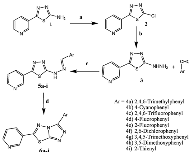
Scheme 1. Reaction sequence for the synthesis of aldehyde hydrazones ( 5a-i ), and 3-substituted-6-(pyridine-3-yl)-[1,2,4]triazolo[3,4-b][1,3,4]thiadiazoles ( 6a-i ).
