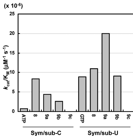
Figure 5. Incorporation efficiencies ( k_{cat}/K_M from steady-state kinetics) of RTP and analogues into sym/sub-C and sym/sub-U.
