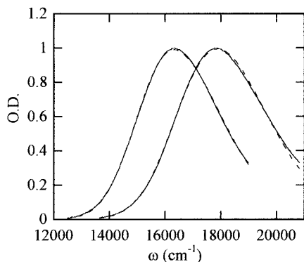
Figure 3. Examples of the fitting of the absorption spectra; left: in methanol, right: in \text{CF}_3\text{H} (2.00). The observed and the fitted spectra are drawn by the solid and the broken lines, respectively.
