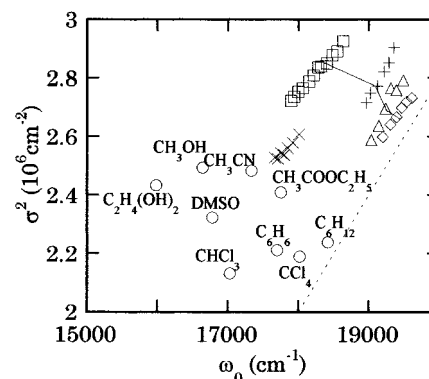
Figure 4. The relation between the first-order ( \omega_0 ) and the second-order ( \sigma^2 ) cumulants of absorption spectra. \circ , in liquid solvents; \square , in \text{CF}_3\text{H} (1.00~2.57) at 50 °C; \times , in \text{CF}_3\text{H} (2.20~2.80) at 10 °C; + , in \text{CO}_2 (1.00~1.90); \triangle , in \text{N}_2\text{O} (1.00~1.98); \diamond , in ethane (1.00~2.00). In each supercritical fluid, \omega_0 is smaller at the higher density. Data points in supercritical fluids at \rho_r = 1.60 are united by the solid line. The dotted line is explained in section 5.
