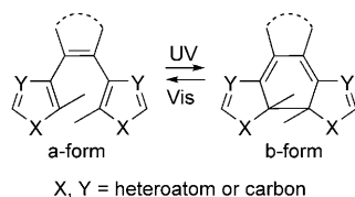
Scheme 1. Photochromism of diarylethene.
