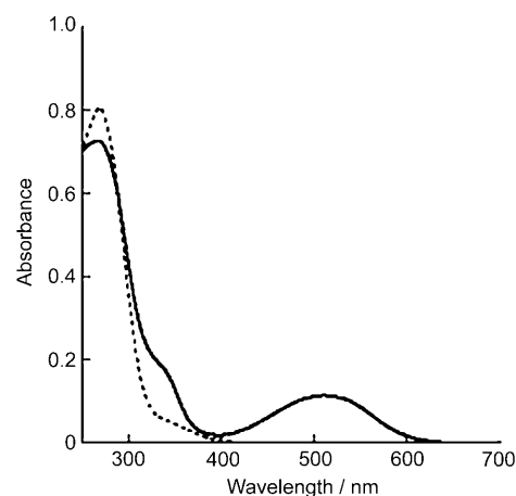
Figure 1. Absorption spectral change of 1 in MeTHF solution ( [1] = 3.3 \times 10^{-5} M): open-form 1a (dotted line) and photostationary state under irradiation with 313 nm light (solid line).
