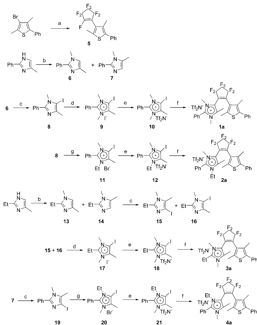
Scheme 4. Synthesis of imidazolium-substituted diarylethenes 1–4 . Reagents: a) 1. n BuLi, 2. perfluorocyclopentene; b) CH 3 I, t BuOK, [18]crown-6; c) I 2 , H 3 IO 6 ; d) CH 3 I; e) LiTf 2 N; f) n BuLi; g) CH 3 CH 2 Br.
