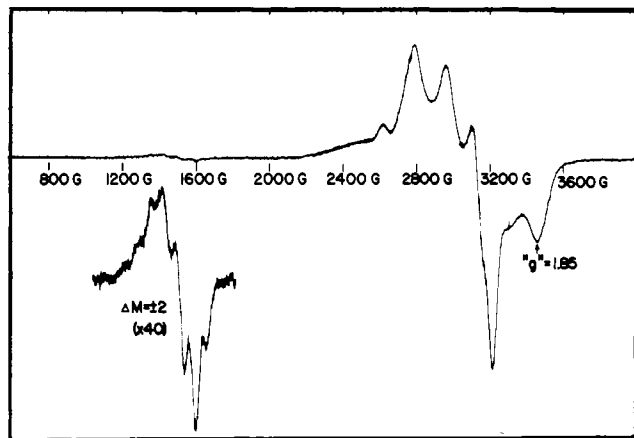
Figure 6. Electron spin resonance spectrum of a frozen 10 mM solution of [\text{Cu}(\text{pip})]_2(\text{im})(\text{NO}_3)_2 \cdot 2.5\text{H}_2\text{O} in \text{Me}_2\text{SO}-\text{H}_2\text{O} (1:1, v/v) at 77 K. The pH of the aqueous solution before addition of the \text{Me}_2\text{SO} was 8.9. Spectrometer settings: 9.108-GHz irradiating frequency, 10-mW microwave power, receiver gain of 800 (32 000 for the half-field transitions), modulation frequency of 100 kHz, modulation amplitude of 5 G, scan rate of 4.2 G/s, and a time constant of 0.3 s.
