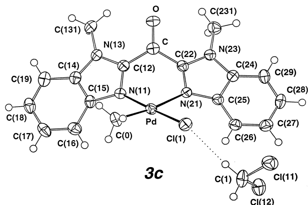
Fig. 5. Projection of 2d and 3c with their associated solvent molecules. Fifty percent displacement ellipsoids are shown for their non-hydrogen atoms having arbitrary radii of 0.1 Å.
