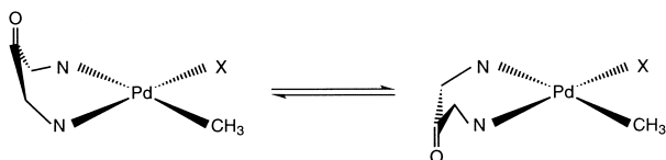
Fig. 7. Fluxional boat-to-boat inversion of the chelate ring in 4b .
